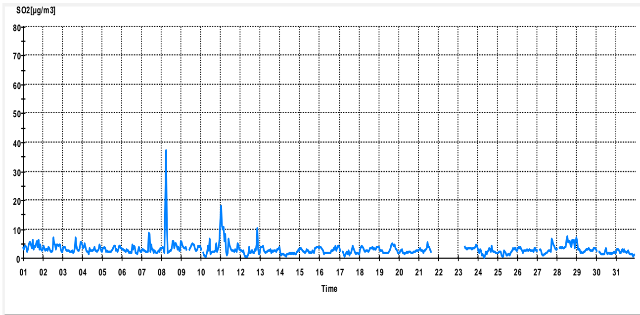
SO2[µg/m3] Monthly Report Terveyskeskus 05.2011 Interval 1 Hour
