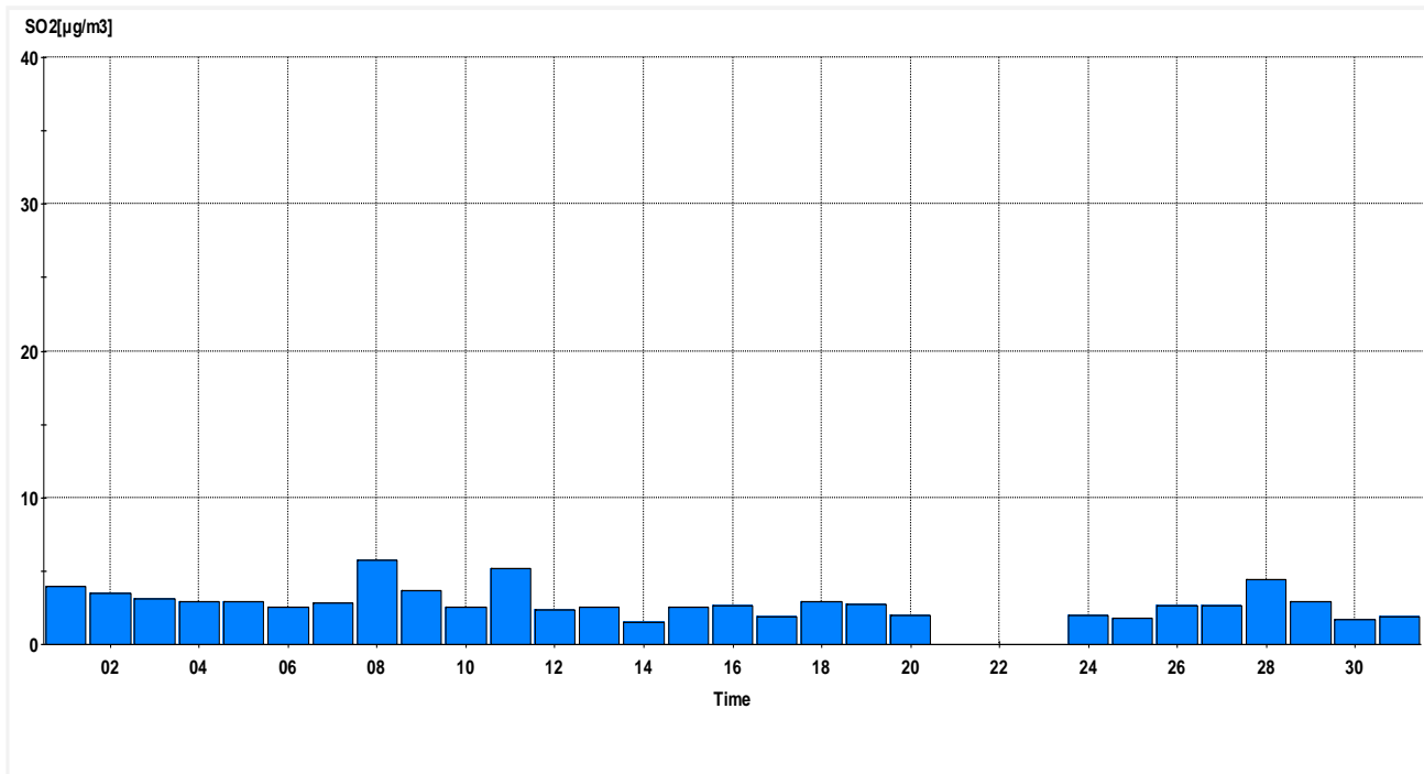
SO2[µg/m3] Monthly Report Terveyskeskus 05.2011 Interval 24 Hour
