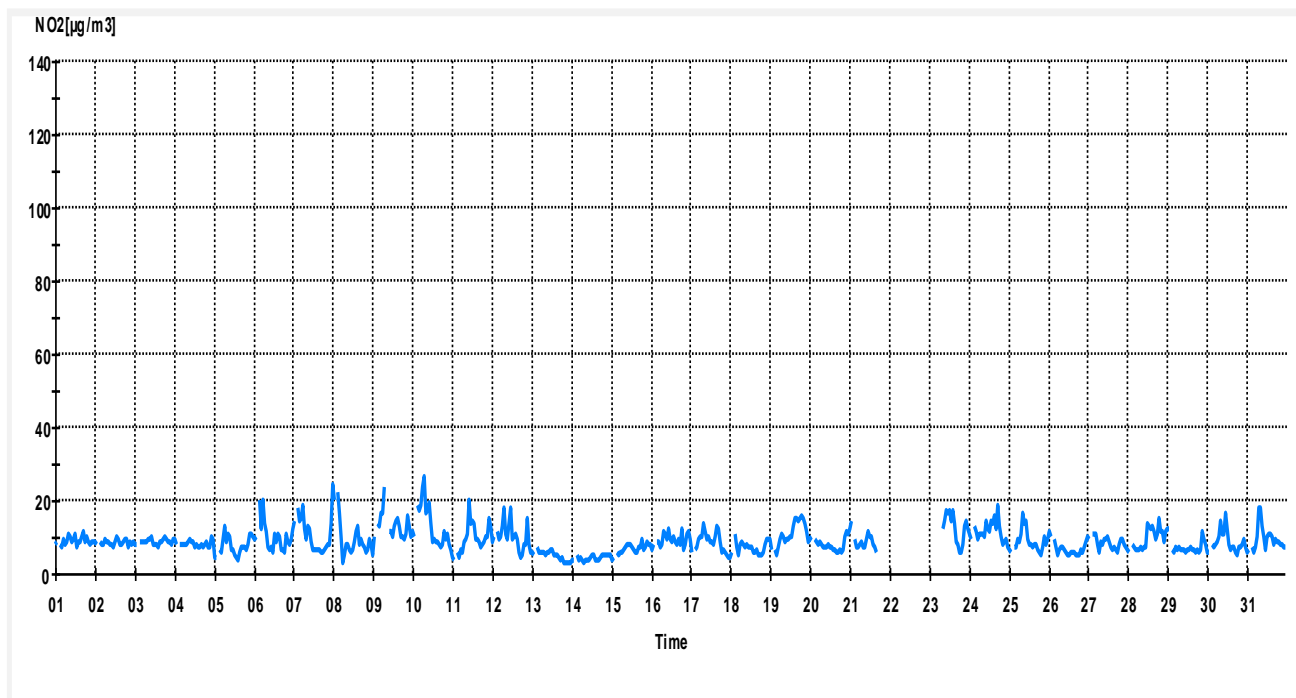
NO 2 [ \mu\text{g}/\text{m}^3 ] Monthly Report Terveyskeskus 05.2011 Interval 24 Hour
