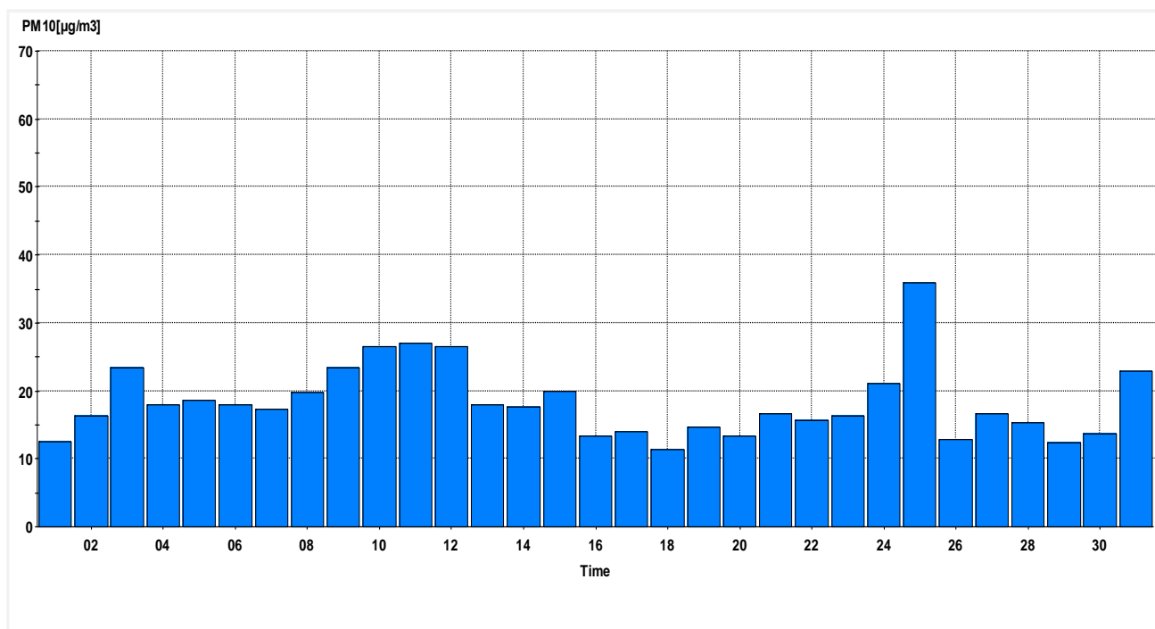
PM10[ \mu\text{g}/\text{m}^3 ] Monthly Report Tekonurmi 05.2011 Interval 24 Hour
