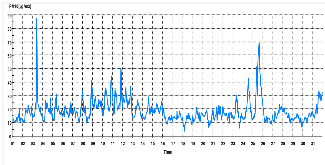
PM10[ \mu\text{g}/\text{m}^3 ] Monthly Report Tekonurmi 05.2011 Interval 1 Hour
