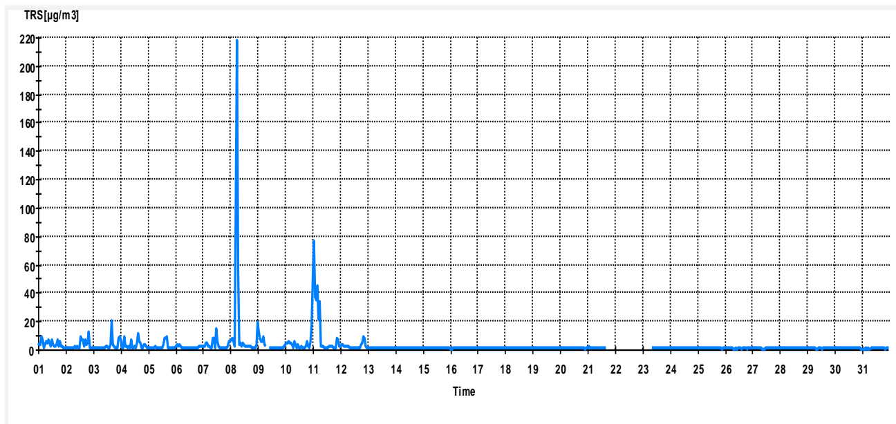
TRS[ \mu\text{g}/\text{m}^3 ] Monthly Report Terveyskeskus 05.2011 Interval 1 Hour
