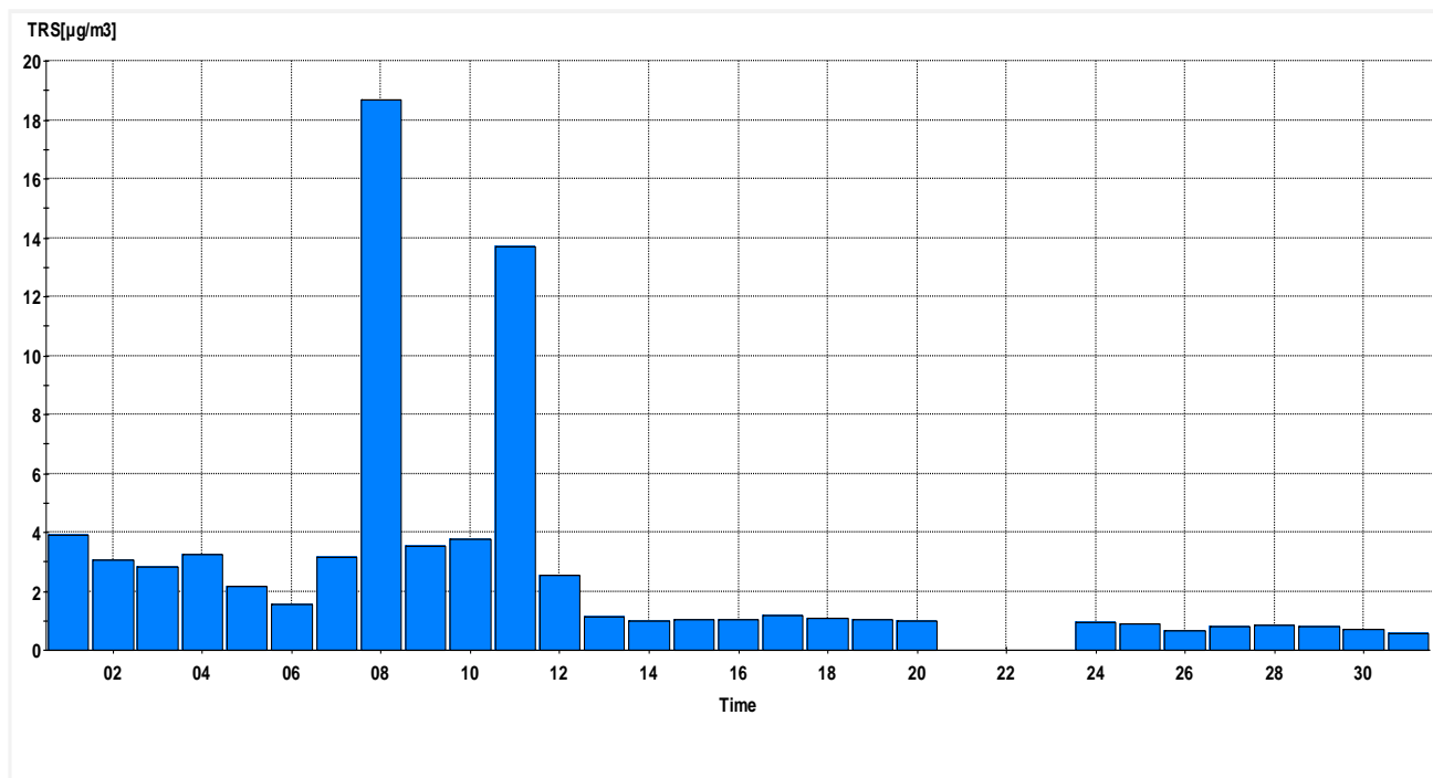
TRS[ \mu\text{g}/\text{m}^3 ] Monthly Report Terveyskeskus 05.2011 Interval 24 Hour
