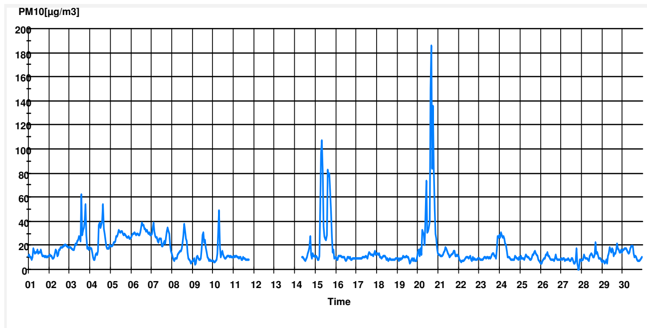
PM10[ \mu\text{g}/\text{m}^3 ] Monthly Report Tekonurmi 11.2011 Interval 1 Hour
